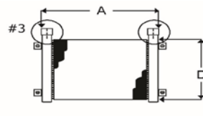
Copper Tubes / Alum Fins / Steel Man (Fixed Brackets)
