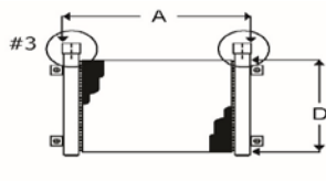
#3 Copper Tubes / Alum Fins / Steel Man (Fixed Brackets)
