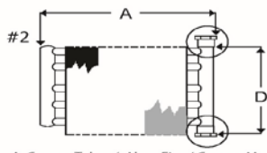
A. Copper Tubes / Alum Fins / Copper Man (Mounting Hardware Included) B. Copper Tubes / Alum Fins / Steel Man (Fixed Brackets)
