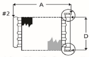
A. Copper Tubes / Alum Fins / Copper Man (Mounting Hardware Included) B. Copper Tubes / Alum Fins / Steel Man (Fixed Brackets)
