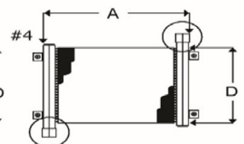
#4 Copper Tubes / Alum Fins / Steel Man (Fixed Brackets)
