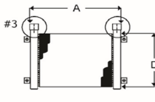
#3 Copper Tubes / Alum Fins / Steel Man (Fixed Brackets)
