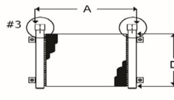
#3 Copper Tubes / Alum Fins / Steel Man (Fixed Brackets)
