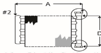
#2 A. Copper Tubes / Alum Fins / Copper Man (Mounting Hardware Included) B. Copper Tubes / Alum Fins / Steel Man (Fixed Brackets)
